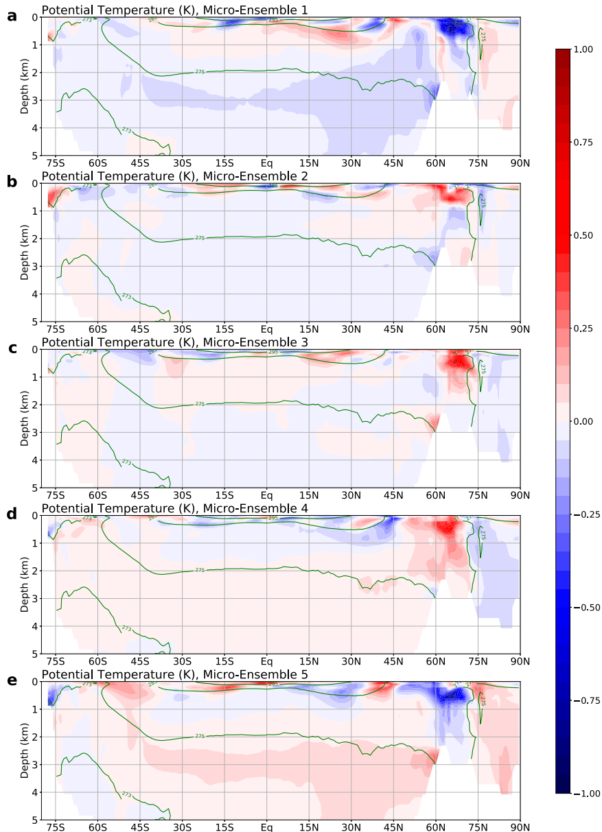
FIG. 2. Zonal-mean ocean potential anomaly (in K; shading) in (a)–(e) microensembles 1–5, respectively, at year 1950 relative to the mean potential temperature (contours at 273, 275, 285, and 295 K) in the full ensemble at year 1950.
