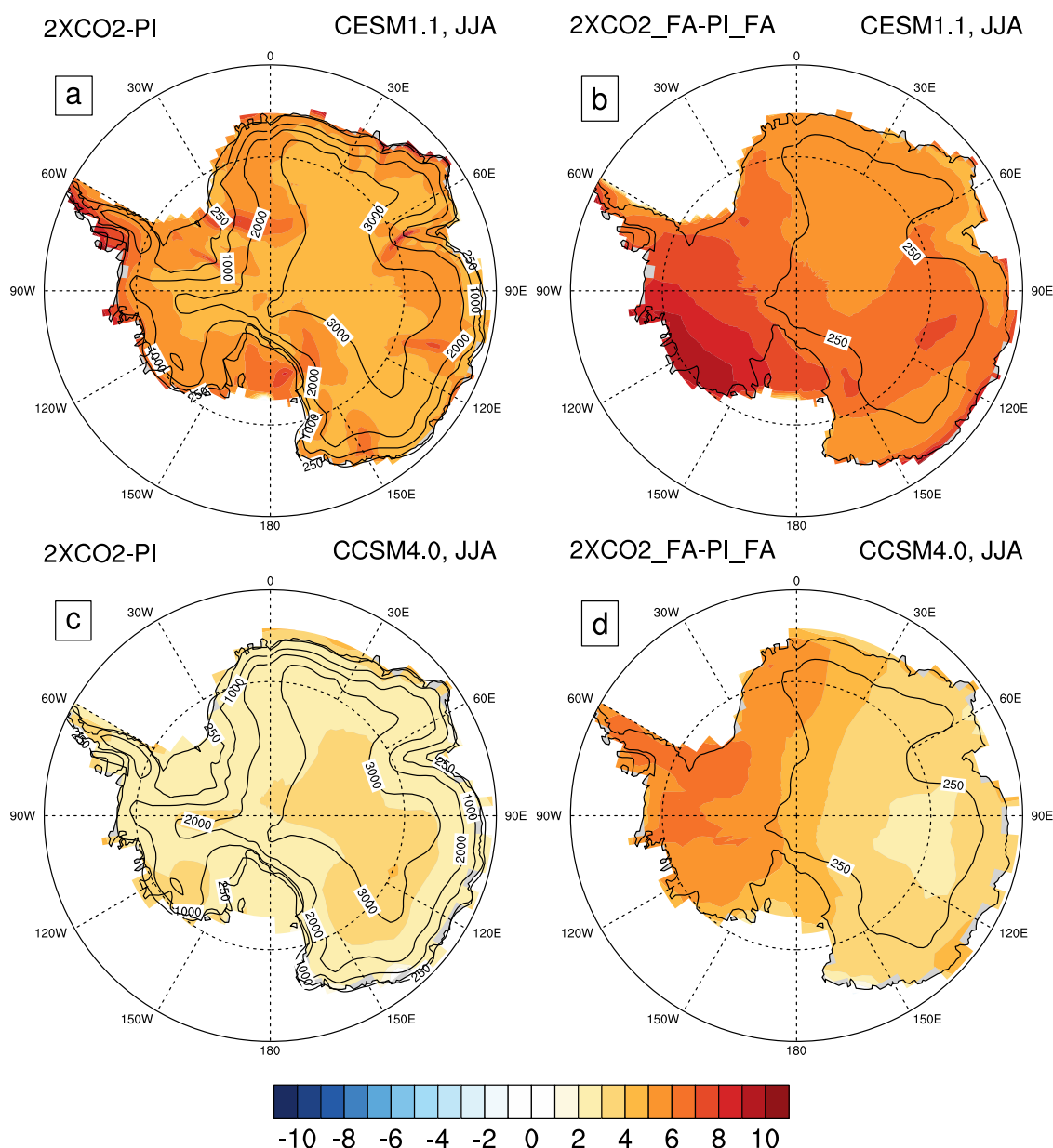
Fig. 3 Antarctic winter season surface temperature change with CO 2 -doubling. Winter season surface temperature change over the Antarctic continent (in K; colors) with CO 2 -doubling in the a, b CESM1.1 and c, d CCSM4.0 when a, c Antarctic orography is at its present-day height, 2 CO 2 minus PI, and when b, d Antarctic orography is flattened to 10% of its present-day height, 2 CO 2 _FA minus PI_FA. Contours show the surface elevation (in m).
