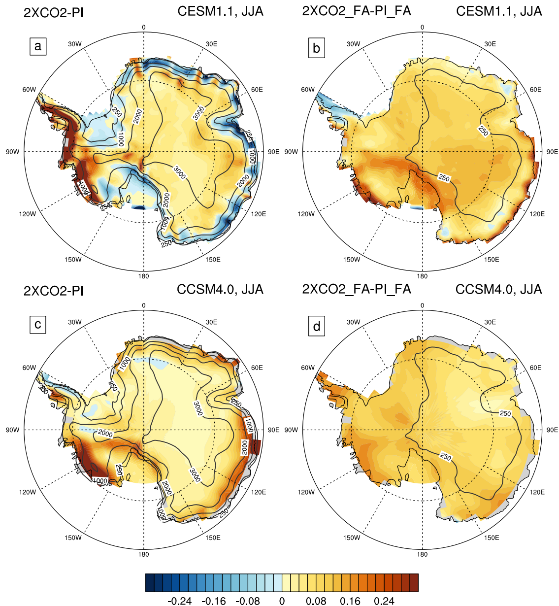
Fig. 6 Condensation heating change with CO 2 -doubling. Change in the lower tropospheric (lowest 200 hPa) condensation heating rate over the Antarctic continent (in K per day; colors) with CO 2 -doubling in the a, b CESM1.1 and c, d CCSM4.0 when a, c Antarctic orography is at its present-day height, 2 × CO 2 minus PI, and when b, d Antarctic orography is flattened to 10% of its present-day height, 2 × CO 2 _FA minus PI_FA. Contours show the surface elevation (in m).
